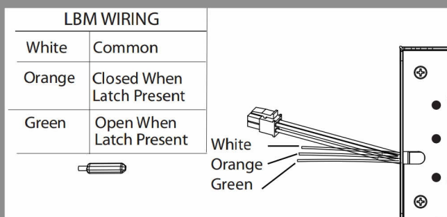
DIAGRAM 3: LATCHBOLT MONITOR
